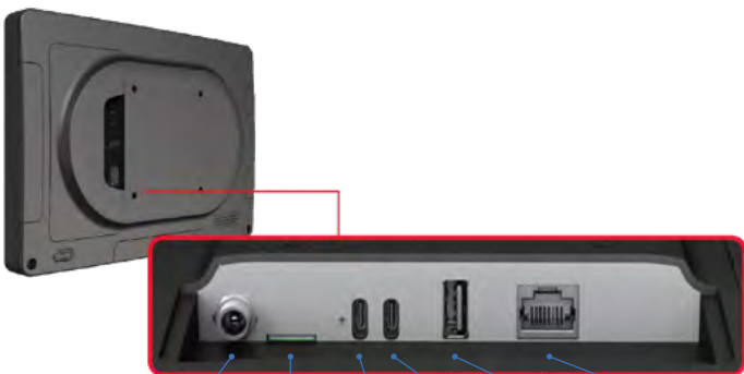
DC-IN Jack SIM USB 3.0 Host USB 2.0 OTG USB 3.0 Type-A RJ45 LAN w/POE
