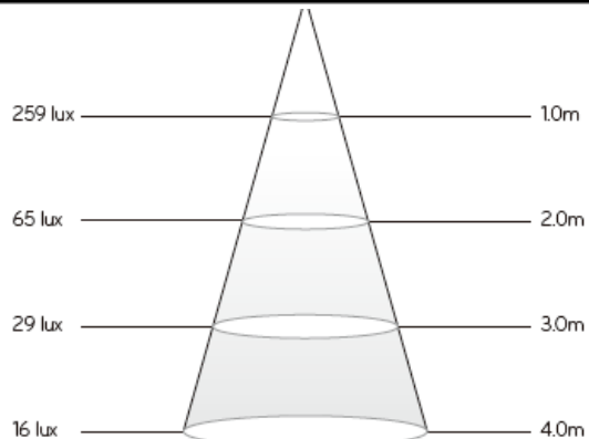
Kegel Lux Diagram/ Cone Lux Diagram
